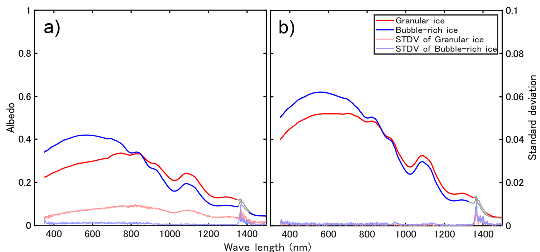
Figure 6. Spectral albedo observed on (a) dark and (b) clean surfaces at ST2c. Red lines indicate the spectral albedo at the surface of the granular ice. Blue lines indicate bubble-rich ice surface removed from surface granular ice. The standard deviations are plotted on the right y-axis using the corresponding light colors. Physical characteristics of granular ice and the amount of LAPs are summarised in Table S1.
