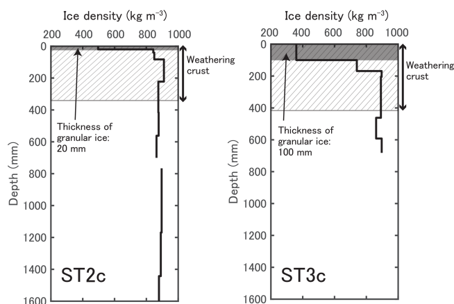
Figure 3. Ice density profile at ST2c (left) and at ST3c (right) at the surface layer. The grey areas indicate layers of weathering granular ice. The weathering crust thickness estimated from ice temperature is indicated by the hatched area.
