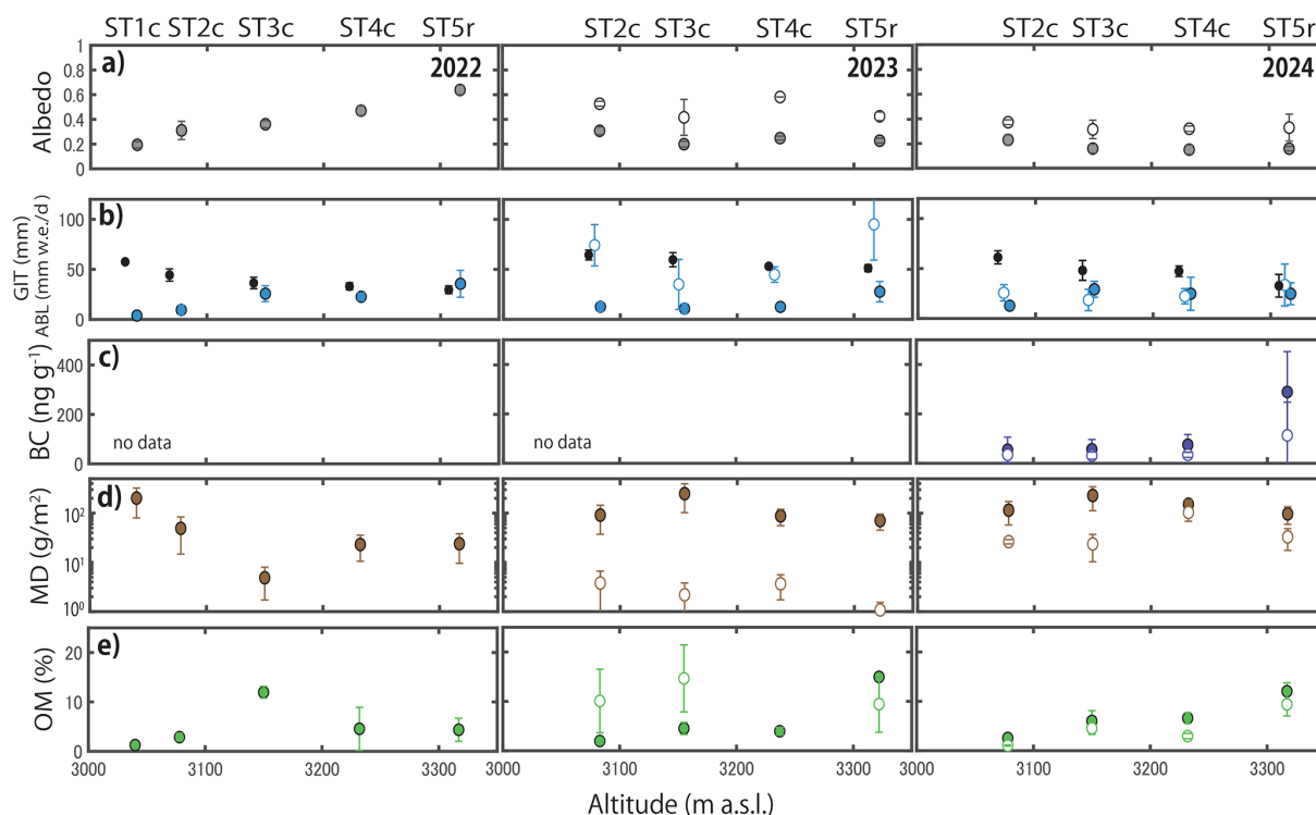
Figure 5. Altitudinal distribution of BB albedo (a), granular ice thickness (GIT), ablation rate (ABL) (b), black carbon (BC) (c), mineral dust (MD) (d), organic matter ratio (OM %) (e). Open circle represents the clean area, while a filled circle indicates the dark area in 2023 and 2024. In panel (b), black circles indicate ABL, and blue open circles and blue filled circles denote GIT in the clean and dark areas, respectively. The vertical axis of MD (d) is logarithmic. Vertical error bars indicate the standard deviations of each multiple measurement. In 2022, sampling was not conducted separately in dark and clean areas. For 2023 and 2024, filled circles represent data from dark surface areas, whereas open circles represent data from clean surface areas.
