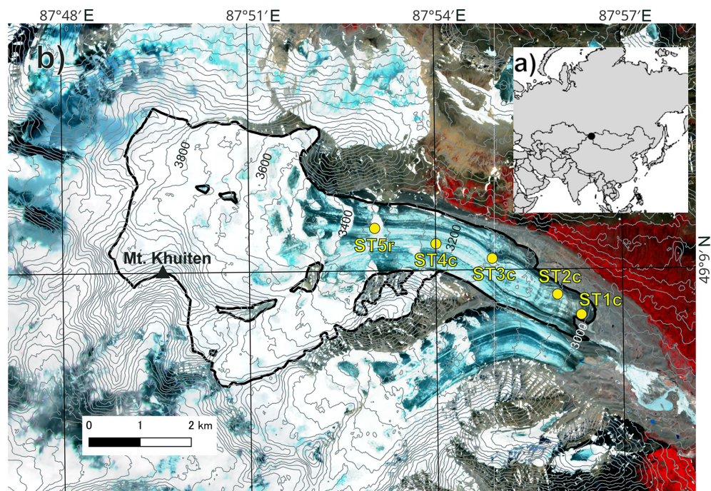
Figure 1. Location map of the Potanin Glacier (a) and observed stake location at the Potanin Glacier (b). The edges of the Potanin glacier are outlined in black. Contour lines are drawn at 50 m intervals. Yellow numbers indicate the location of stake, sampling site. The back satellite imagery is Sentinel 2 (False color) acquired on 15 July 2023.
