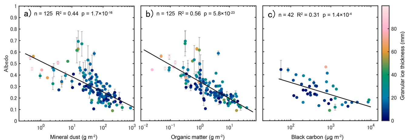
Figure 7. Relation between BB albedo and particles (MD, OM, BC) a)–c). The colour of the circle indicates surface granular ice thickness. All horizontal axes are logarithmic.
