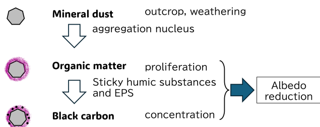
Figure 11. Schematic diagram showing the relationship between the three major LAPs (MD, OM, BC).
