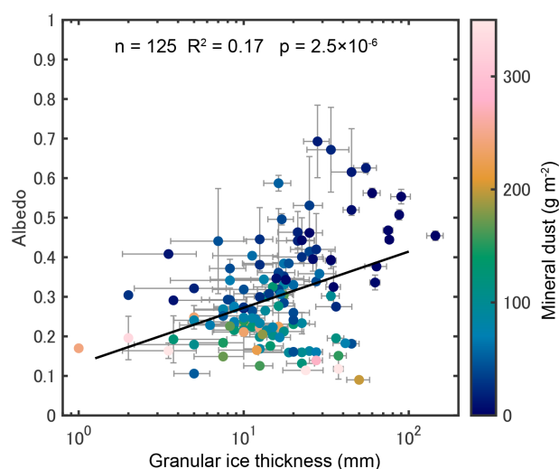
Figure 8. Relation between BB albedo and granular ice thickness (GIT). The circle colour indicates the amount of mineral dust per area.
