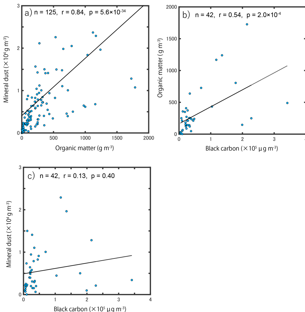
Figure 10. Relationships among the concentrations of the three major light-absorbing particles on the glacier surface: (a) mineral particles and organic matter; (b) black carbon and organic matter; (c) black carbon and mineral particles. Note that black carbon was sampled only in 2024, so there are only 42 samples.
